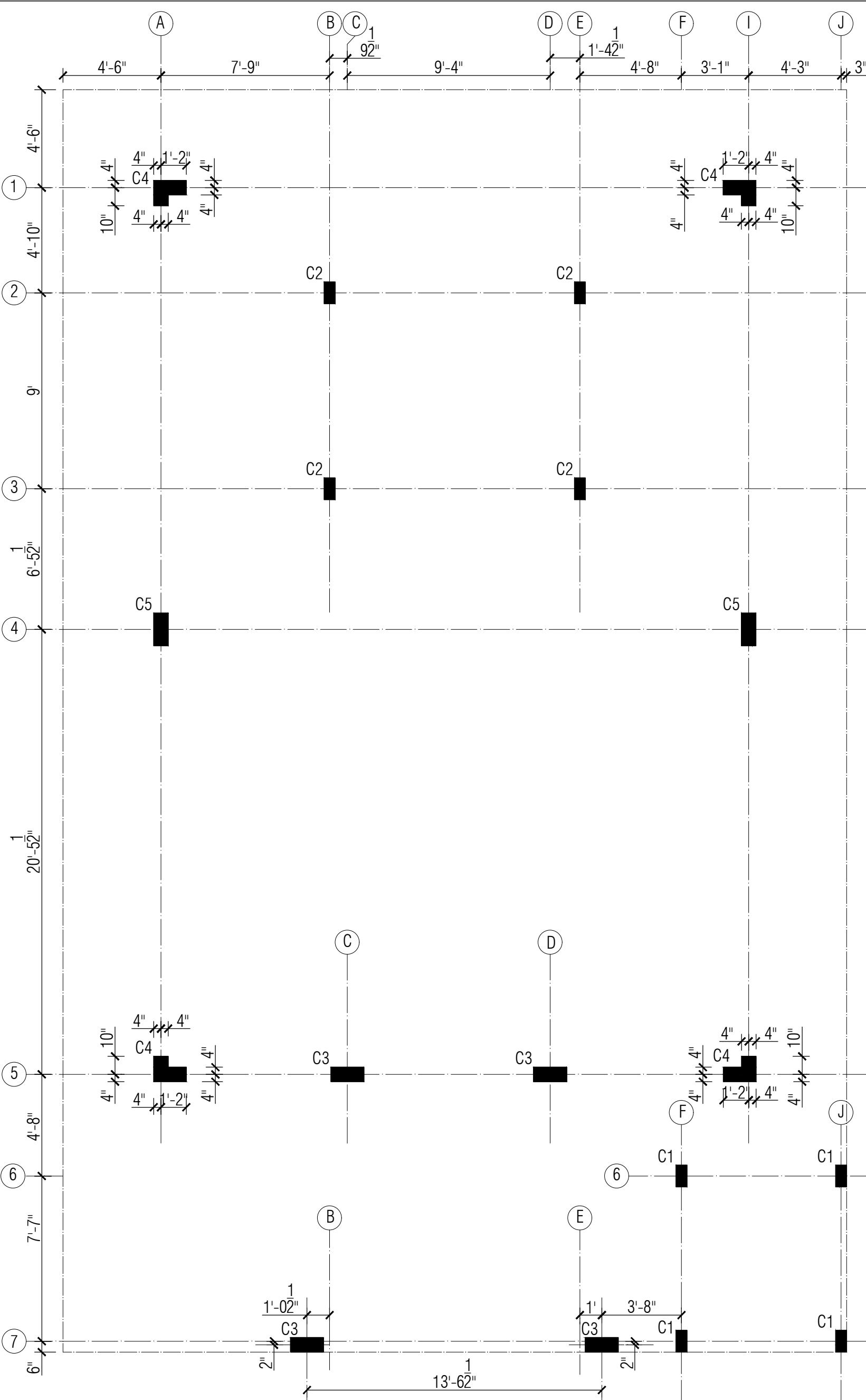
PLAN - COLUMN LAYOUT
